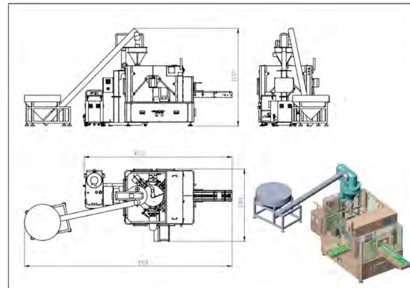
R8-PMPB with screw feeder
