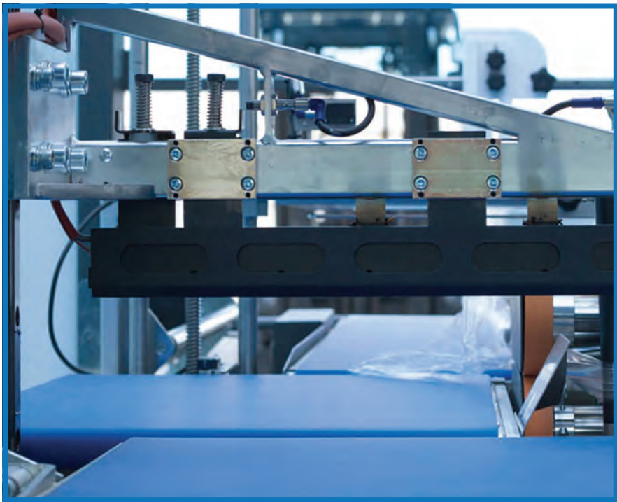
Movable center conveyor belt
